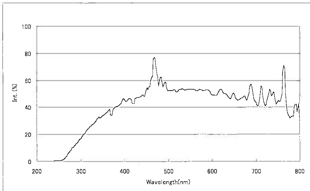
Fig. 2 YXL-2200B2 Spectral Distribution Map
